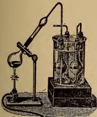
Fig. 85. BUNSEN'S APPARATUS FOR OBTAINING VOLUME OF CHLORINE (gas).
